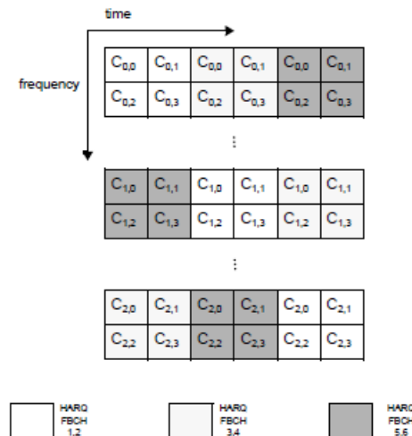
Figure 558—2x2 HMT structure
